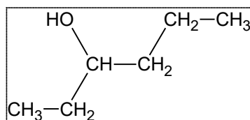
(19) Hexan-3-ol
