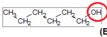
alcool: hexan-1-ol
