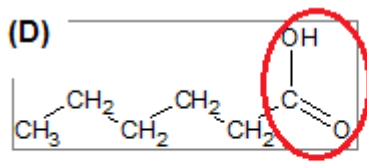
acide carboxylique
