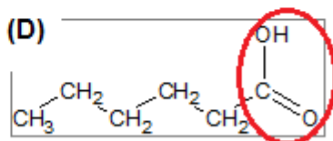
acide carboxylique
