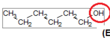
alccool: hexan-1-ol
