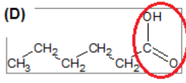
acide carboxylique
