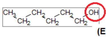
alcool: hexan-1-ol
